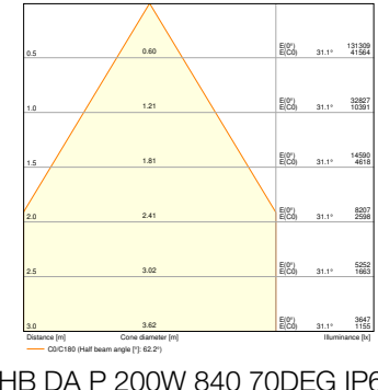
HB DA P 200W 840 70DEG IP66 WITH REFRACTOR
