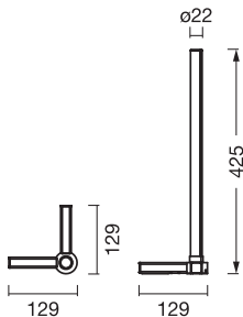
SMART WIFI CORNER TABLE MGC RGBBK
