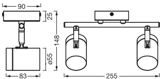
LED SPOT STAMP 2XGU10 WT
