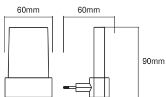
Produkt Line Drawing LUNETTA Shine WT
