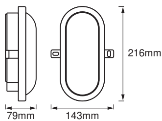
LED BULKHEAD 12W
